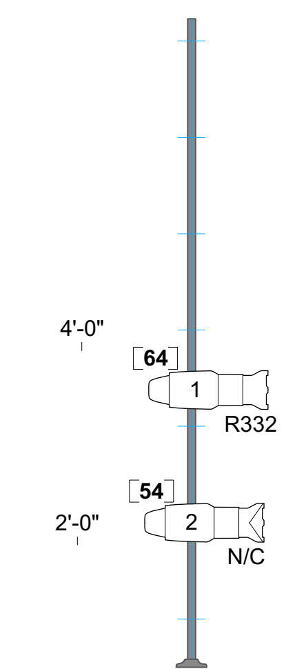
SR Boom 3 Notes: From Center Line: 19'0" From Plaster Line: 13'6"
