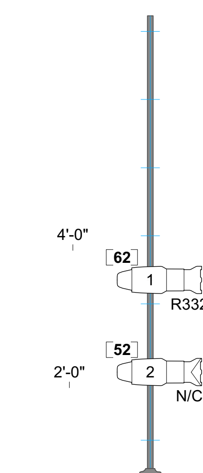
SR Boom 1 Notes: From Center Line: 19'0" From Plaster Line: 3'0"
