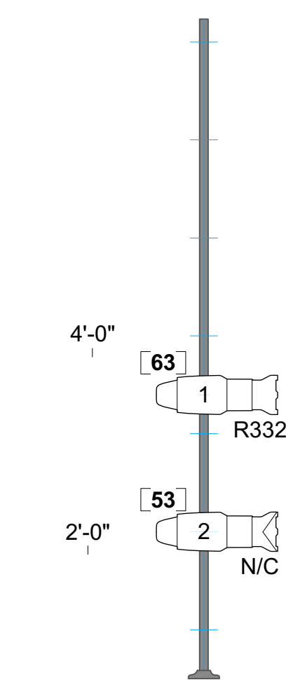
SR Boom 2 Notes: From Center Line: 19'0" From Plaster Line: 9'0"
