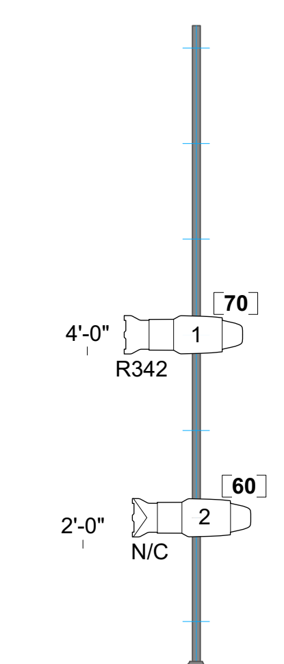
SL Boom 4 Notes: From Center Line: 19'0" From Plaster Line: 19'0"
