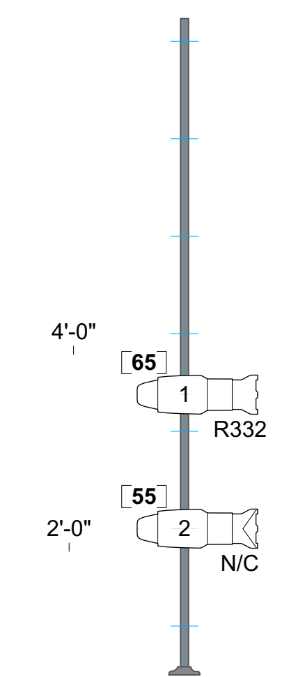
SR Boom 4 Notes: From Center Line: 19'0" From Plaster Line: 19'0"
