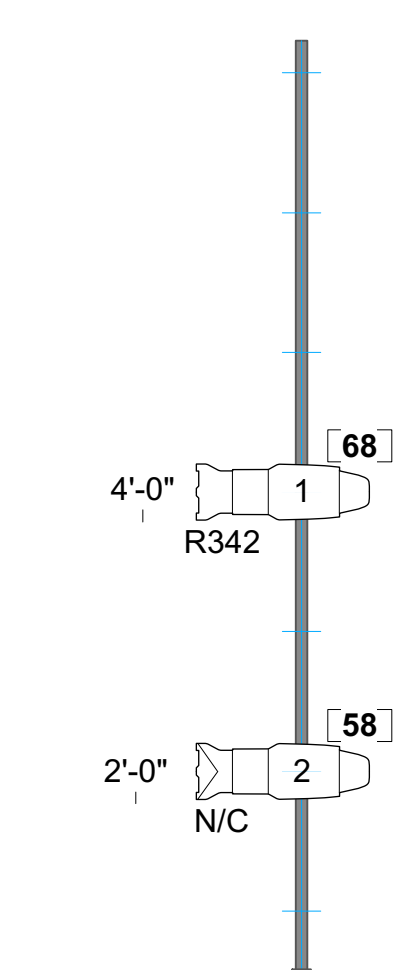
SL Boom 2 Notes: From Center Line: 19'0" From Plaster Line: 9'0"
